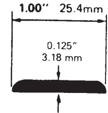
DR1 0.064 kg/ft 0.21 kg/m also DR2 (6082 TF)
