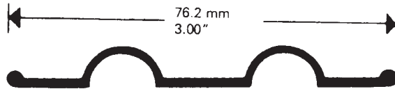
PP2 INTERIOR RUB RAIL 0.132 kg/ft 0.433 kg/m
