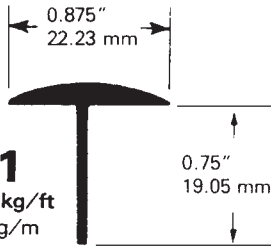
PP2 INTERIOR RUB RAIL 0.132 kg/ft 0.433 kg/m
