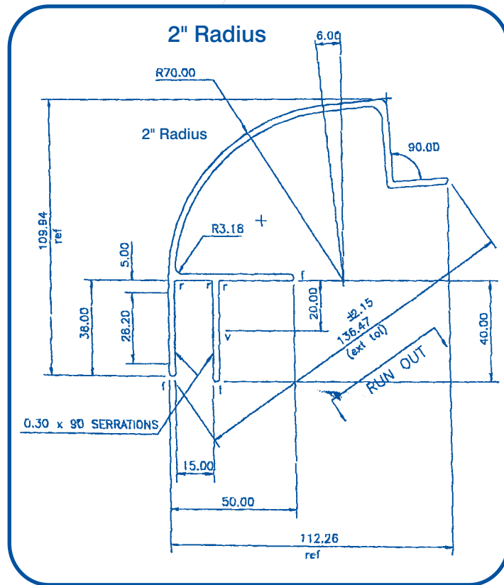
CR25 14mm Captive Cant Rail
